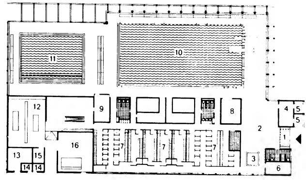
3 Ground floor
